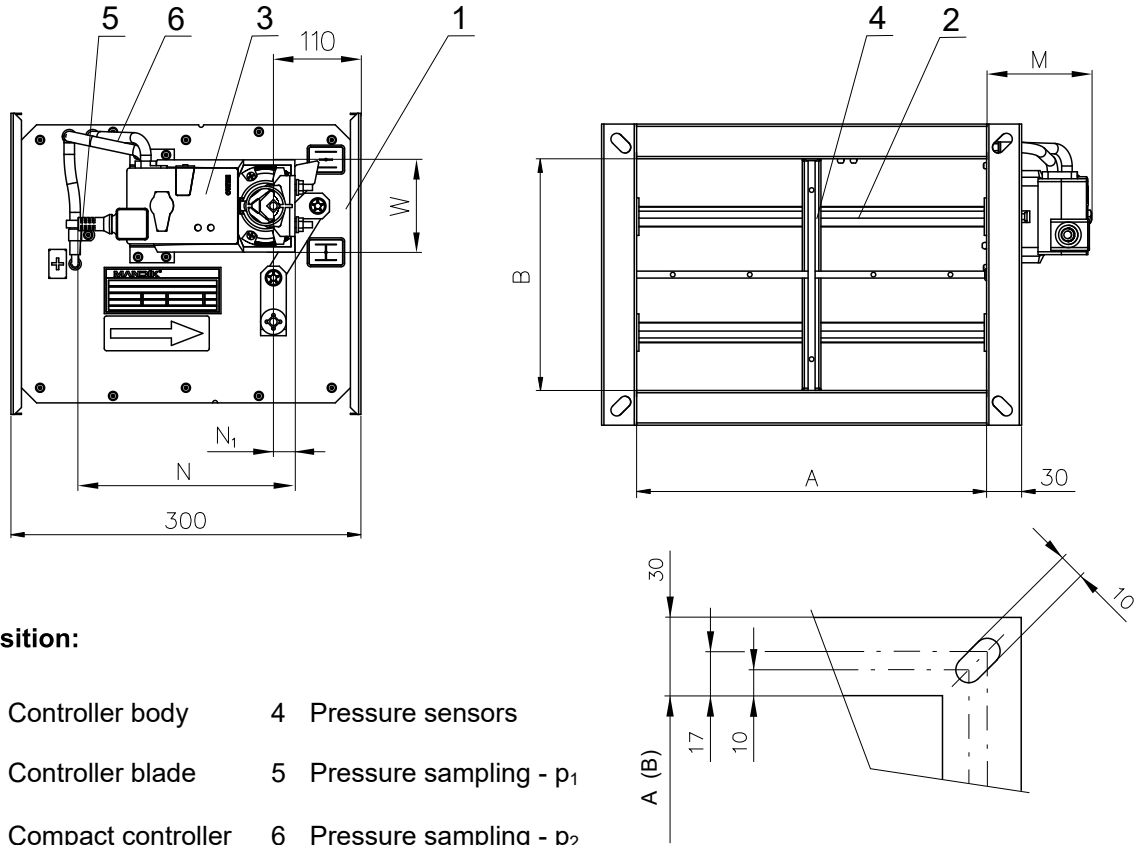
Fig. 31 RPMC-V - with insulation
