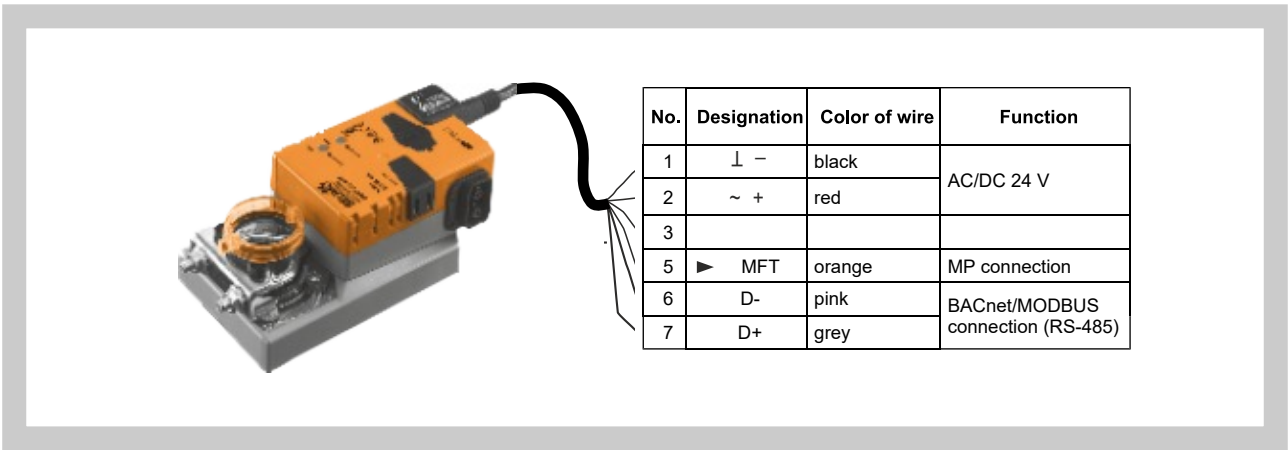
Fig. 9 Actuators LMV-D3-MOD, NMV-D3-MOD and SMV-D3-MOD
