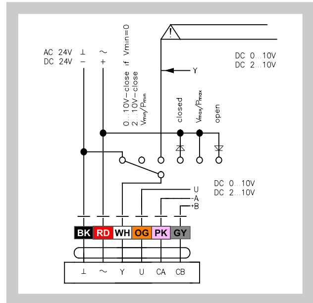
Fig. 21 Regulator 327VM-024-...-MB
