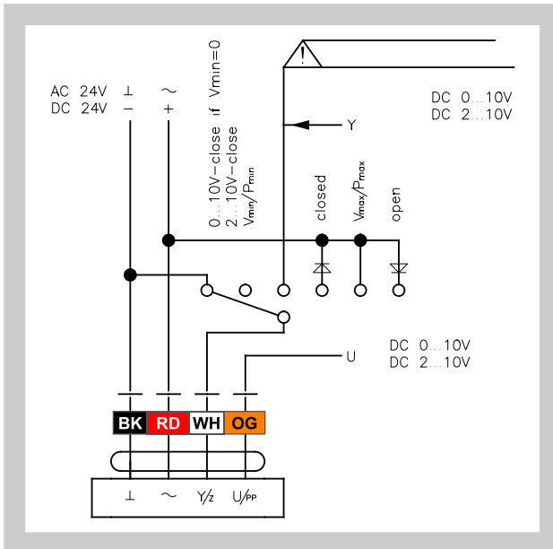
Fig. 20 Regulator 327VM-024-...
