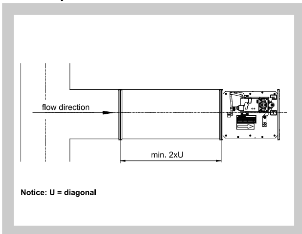
Fig. 32 Recommended distance from double branch joint
