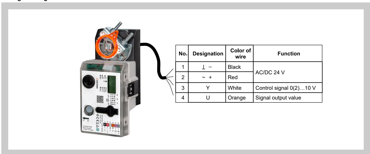
Fig. 19 Regulators 327VM-024-... -MB
