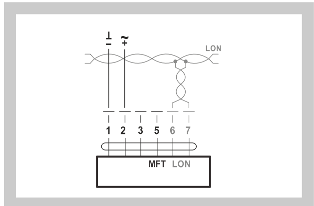
Fig. 13 Wiring of actuators LMV-D3-LON and NMV-D3-LON
