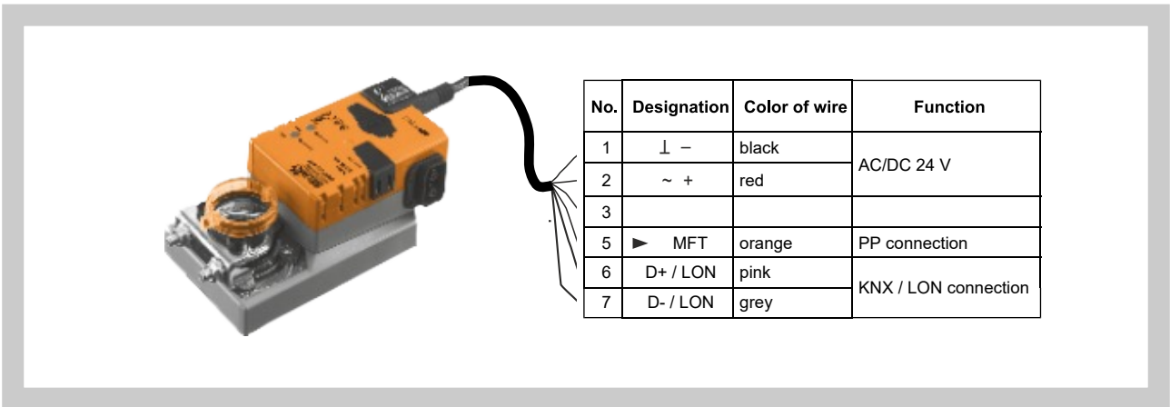
Fig. 11 Actuators LMV-D3-KNX, NMV-D3-KNX, LMV-D3-LON and NMV-D3-LON
